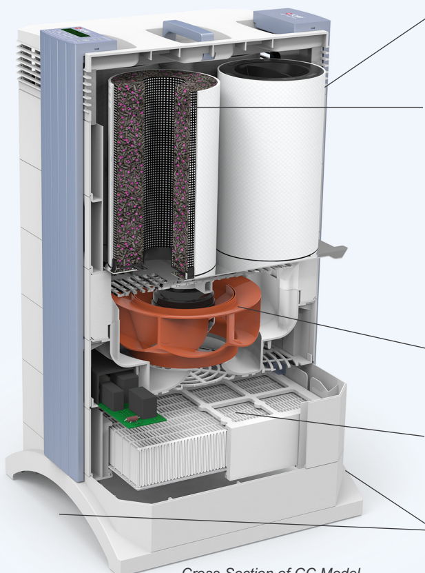
Cross-Section of GC Model
